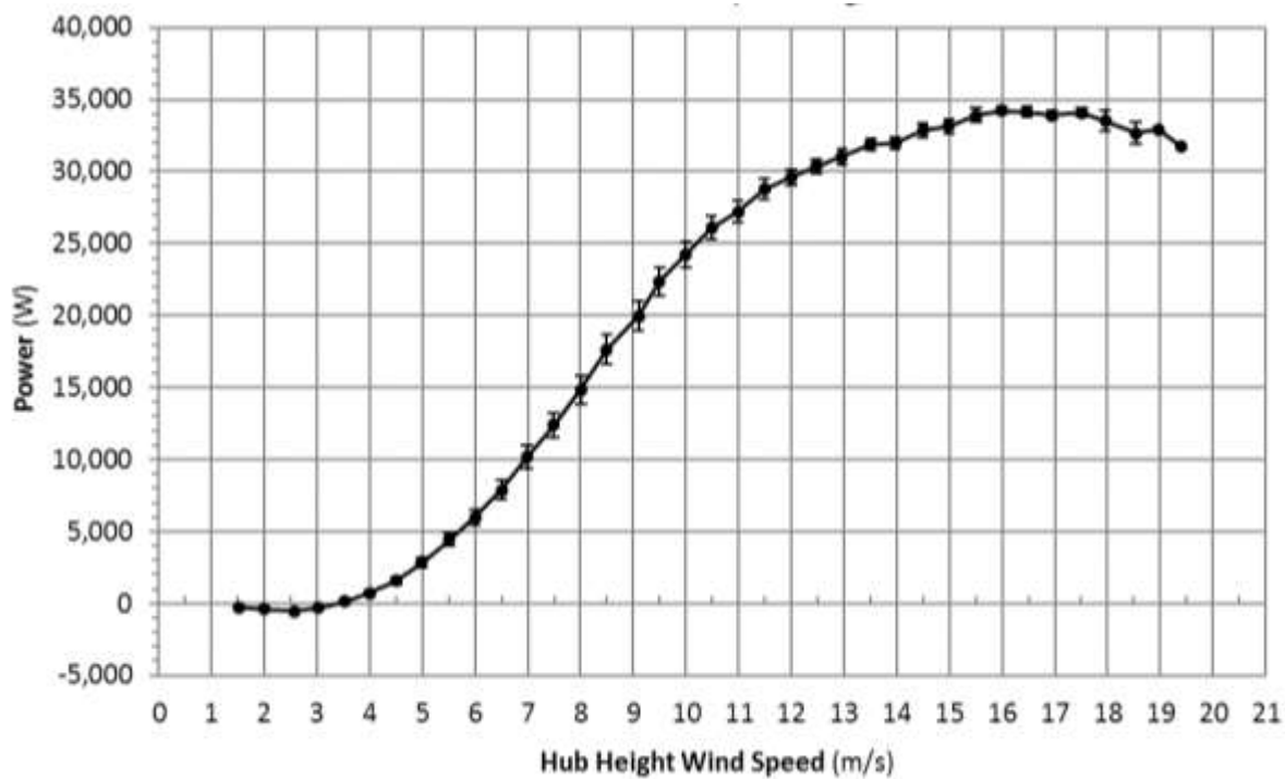
Power Curve with Combined Standard Uncertainty Aircon LA30 Reference air density: 1.225 kg/m 3
